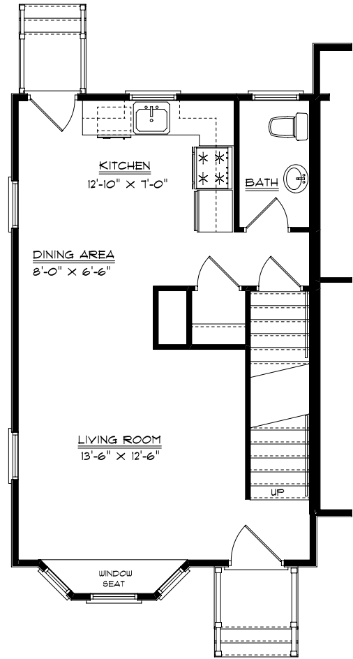
FIRST FLOOR PLAN B UNIT
