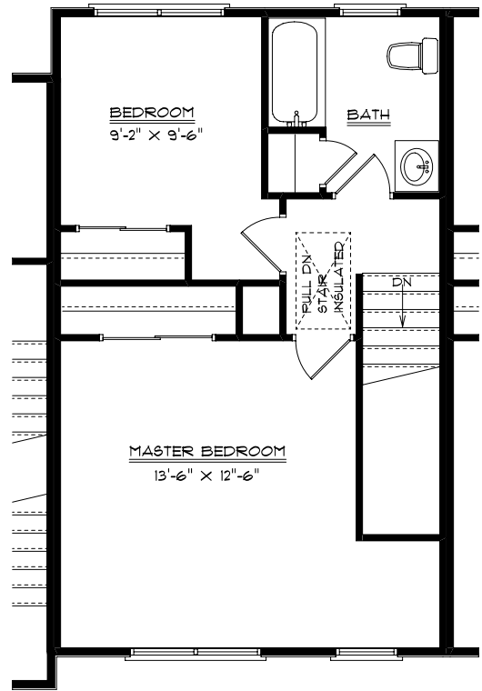
SECOND FLOOR PLAN C UNIT
